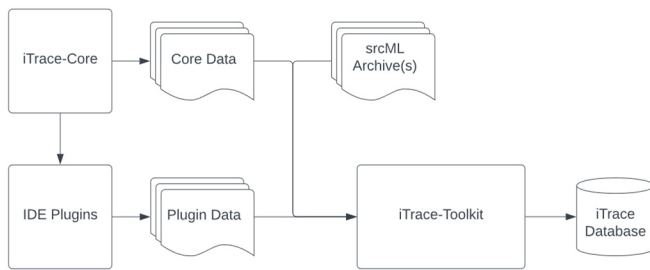
Figure 1: An overview of the iTrace Infrastructure and how iTrace-Toolkit fits within it.
